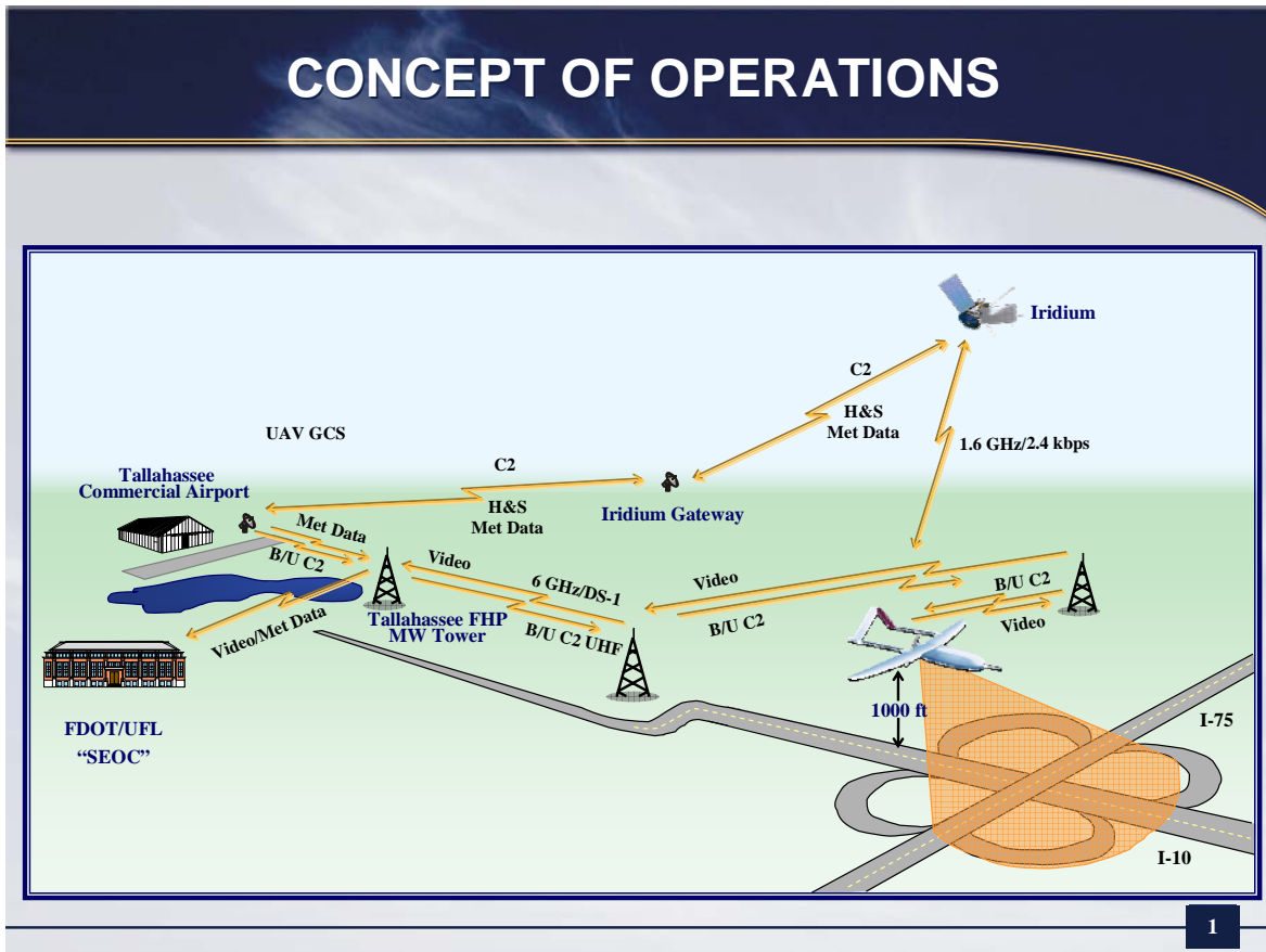
Figure 2. Graphic View of UAV Test Scenario
